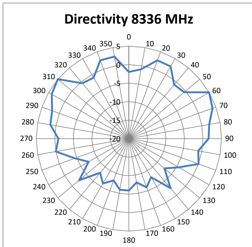
Fig. 10: Directivity plot 8336 MHz
