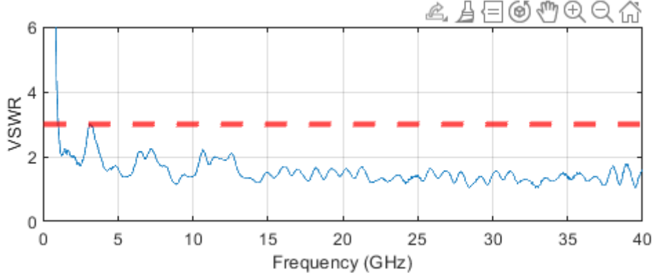
Fig. 13: Broadband matching (newest generation, antenna 2)
