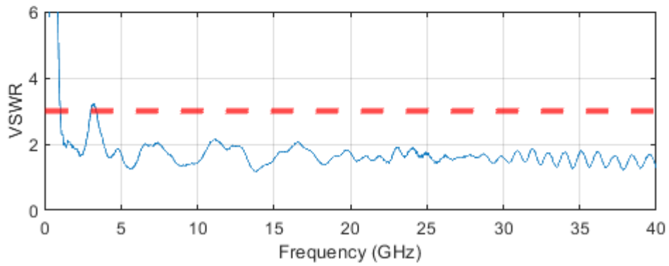
Fig. 13: Broadband matching (newest generation, antenna 1)
